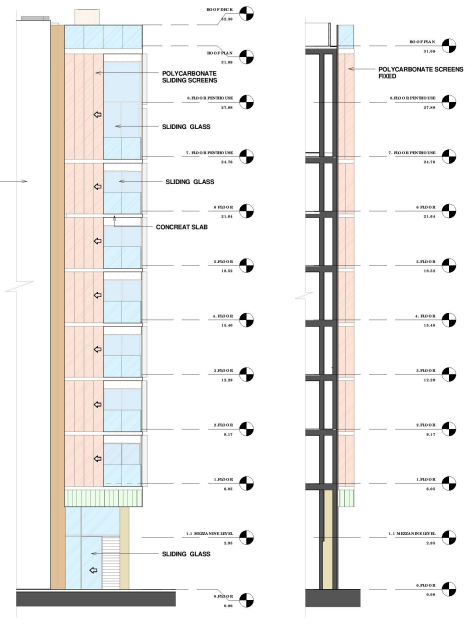
3 ELEVATION SIDE 2 1:100
