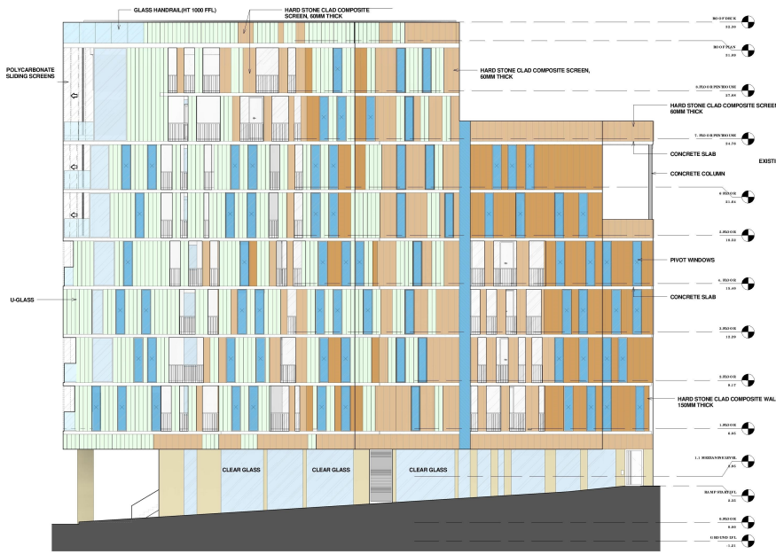
1 ELEVATION SIDE 1:100
