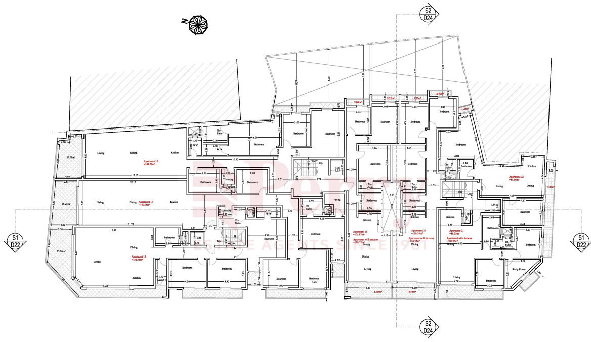
P6 D6 PROPOSED THIRD FLOOR PLAN Scale 1:100
