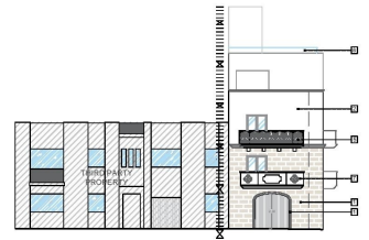
PROPOSED Elevation/Streetscape 1:200
