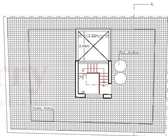
Roof Level Proposed Scale 1:100
