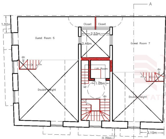
3rd Floor Level (int) Proposed Scale 1:100
