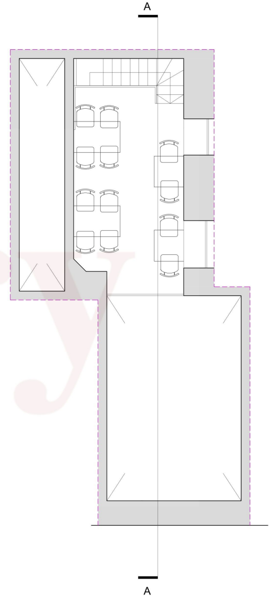
Mezzanine Floor as Proposed Scale 1:50
