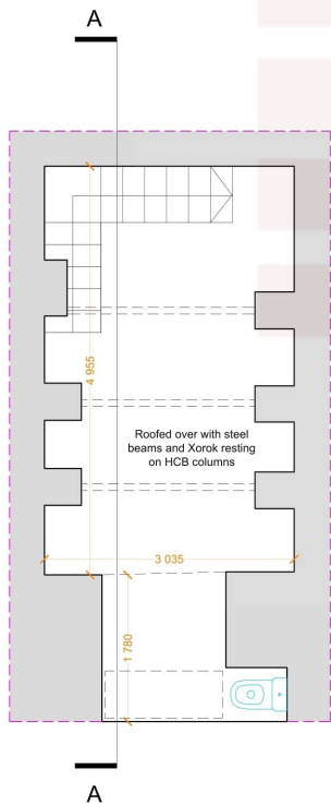
Basement as Existing Scale 1:50
