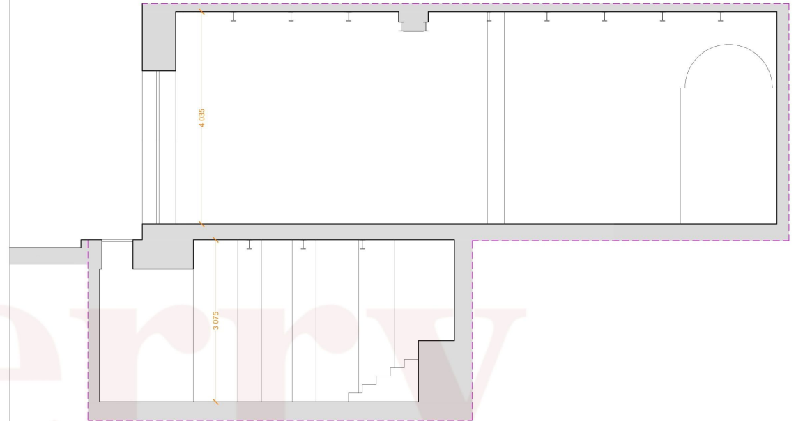
Section A-A as Existing Scale 1:50
