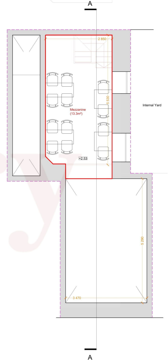
Mezzanine Floor as Proposed Scale 1:50
