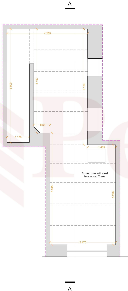
Ground Floor as Existing Scale 1:50
