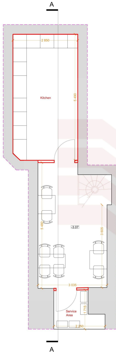
Basement as Proposed Scale 1:50
