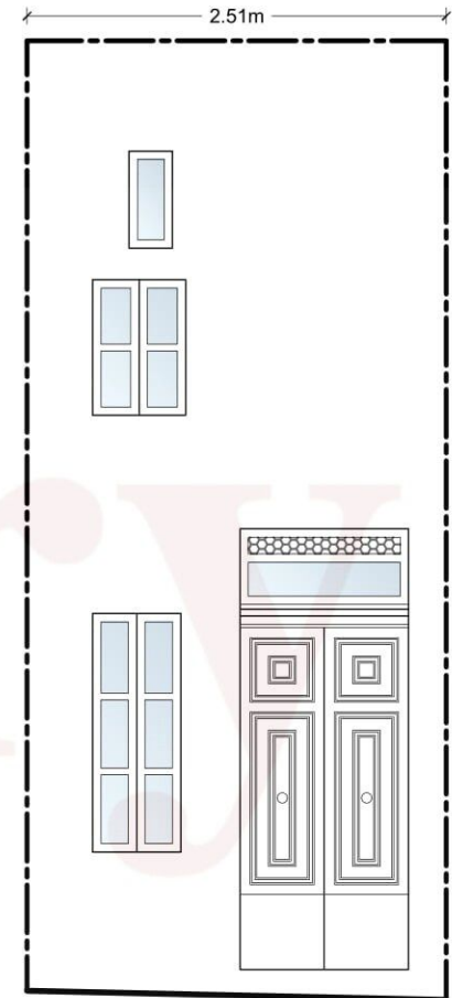
Existing Elevation
