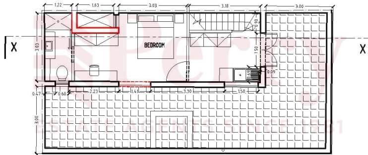
RECESSED FLOOR LEVEL
