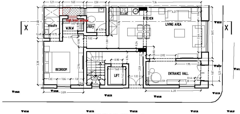
GROUND FLOOR LEVEL
