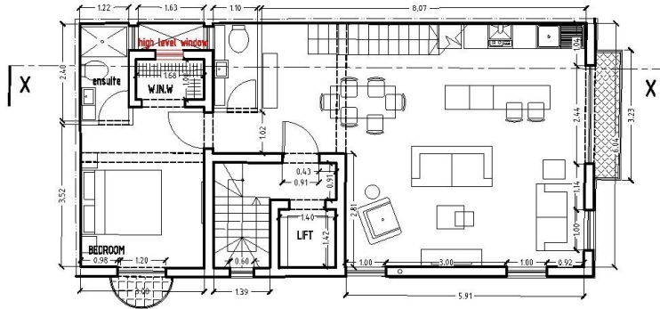
3rd FLOOR LEVEL - duplex
