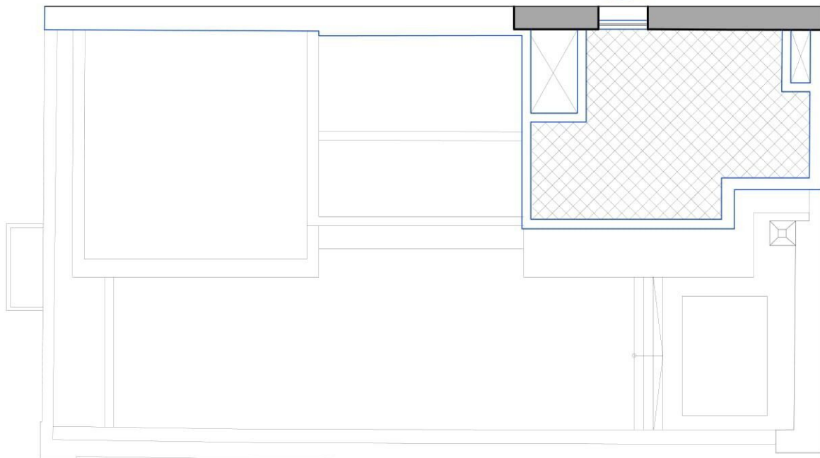
PROPOSED UPPER ROOF Scale:- 1:100 (CLEAN COPY)
