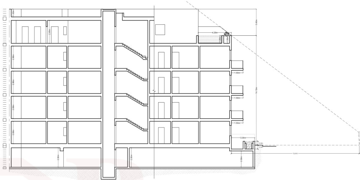
Proposed Section A-A scale 1:100
