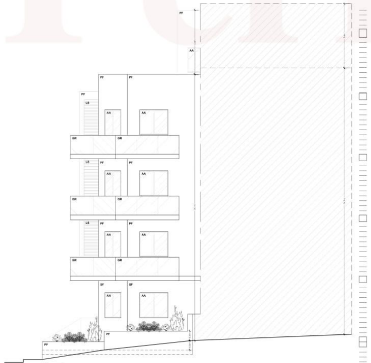
Proposed Side Elevation Scale 1:50
