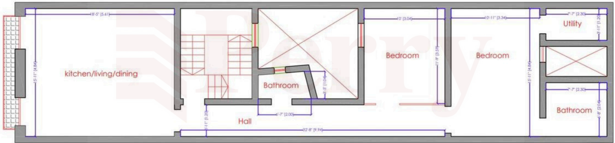
Sketch Layout Plan Scale 1:100
