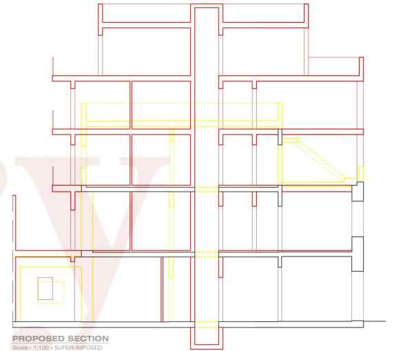
PROPOSED SECTION Scale: 1:100 - SUPER-IMPOSED
