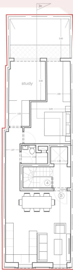
PROPOSED LEVEL 3 Scale: 1:100 - CLEAN COPY
