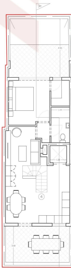
PROPOSED LEVEL 4 Scale: 1:100 - CLEAN COPY
