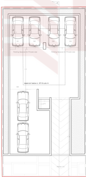
PROPOSED BASEMENT Scale:- 1:100
