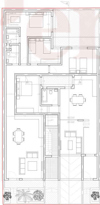
PROPOSED GROUND FLOOR Scale:- 1:100
