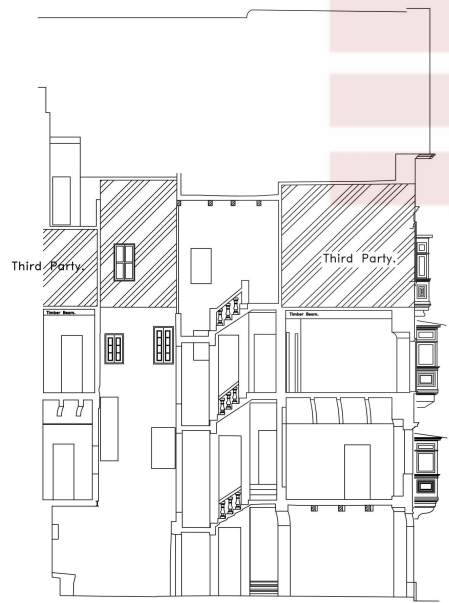
Section A-A Level=28.00m
