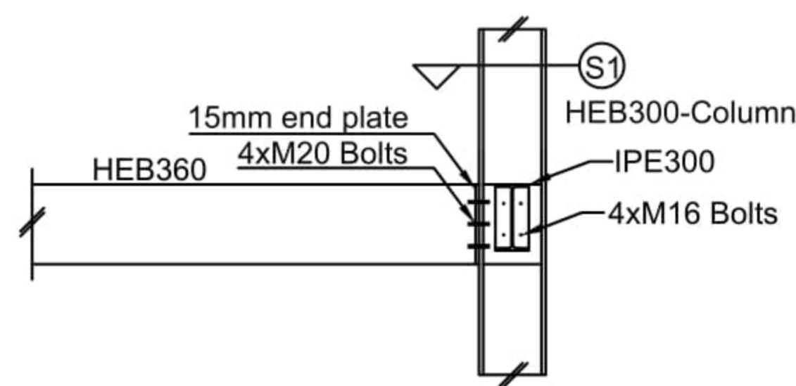
DETAIL 1 scale 1:50
