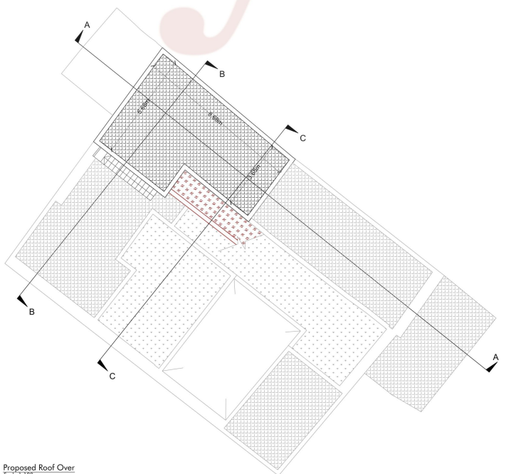
Proposed Roof Over Scale 1:100
