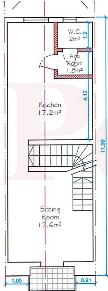
PROPOSED FIRST FLOOR - 50.13m 2 Scale:-1:100
