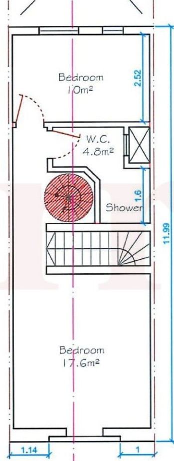
PROPOSED SECOND FLOOR - 50.13m 2 Scale:-1:100
