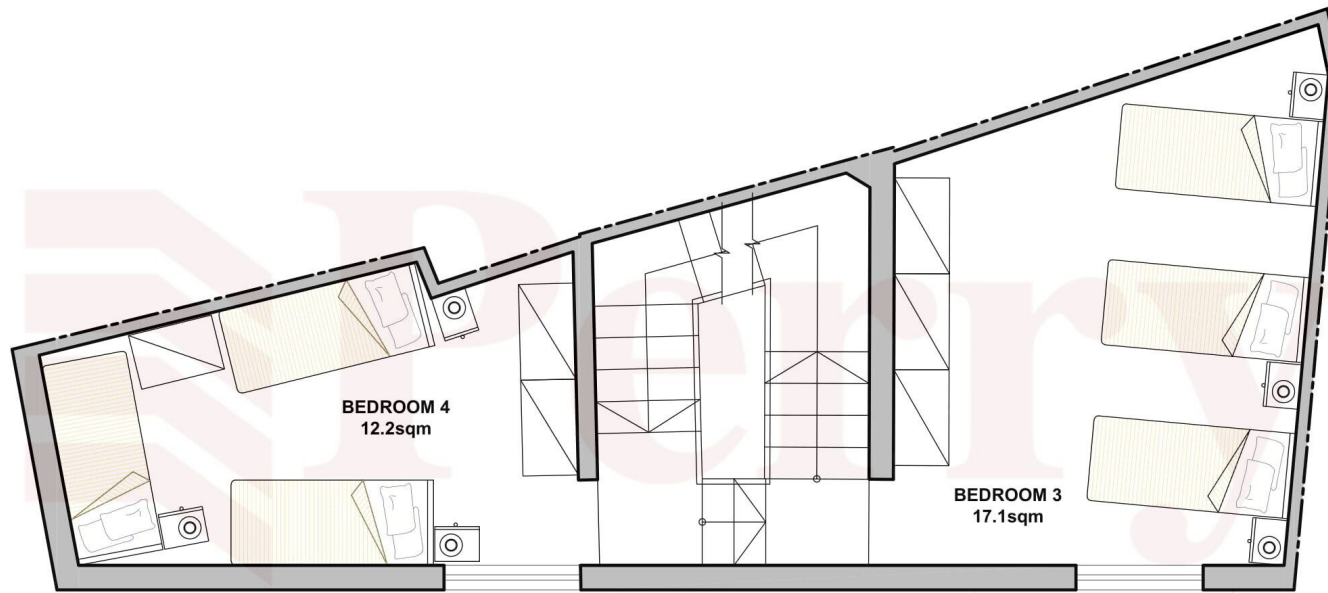
P1 EXISTING SECOND FLOOR PLAN D3 Scale 1:50
