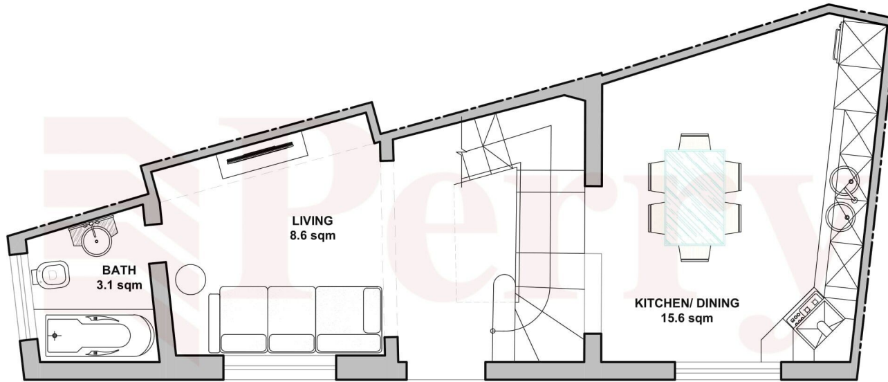
P1 EXISTING GROUND FLOOR PLAN D1 Scale 1:50
