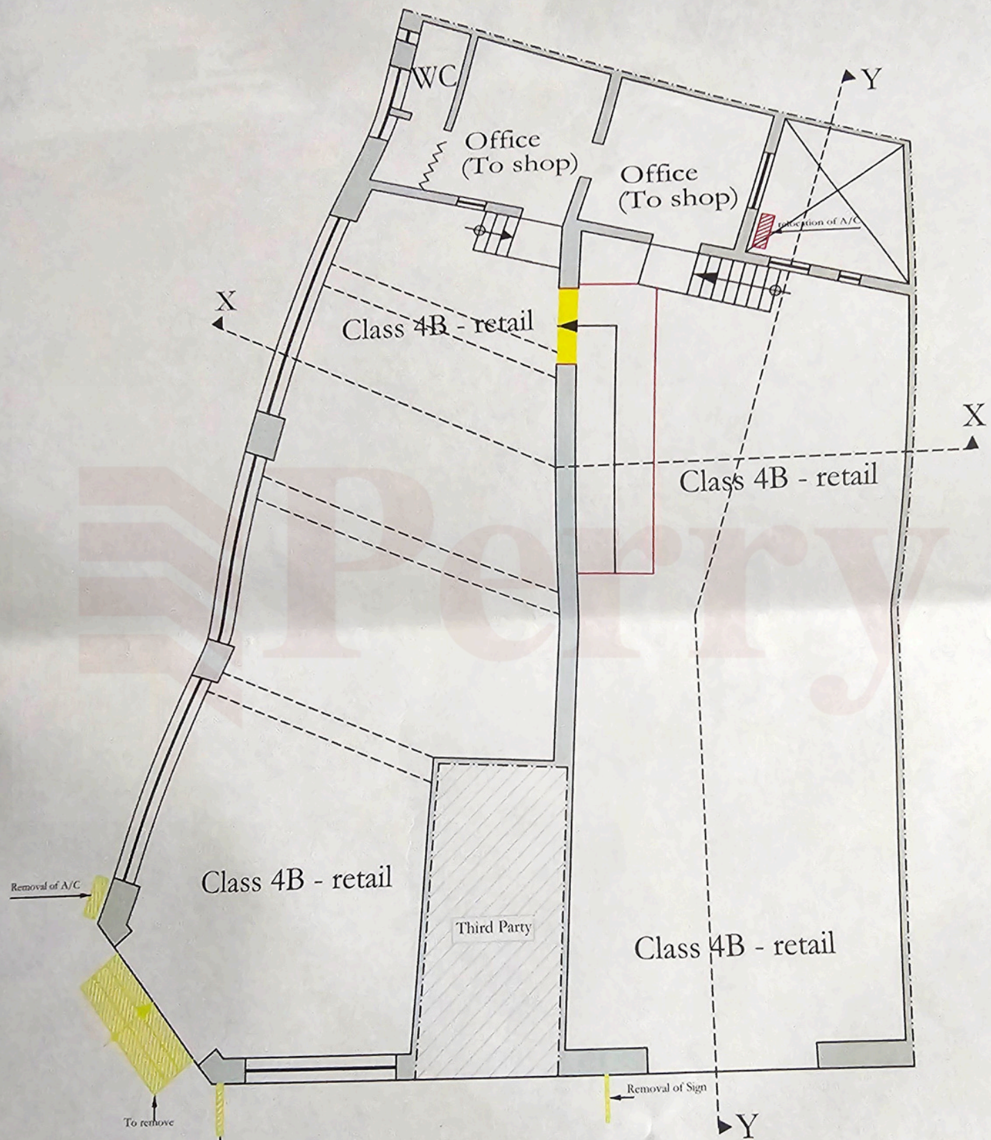
Ground Floor Plan Scale 1:100 Site Area=240m 2
