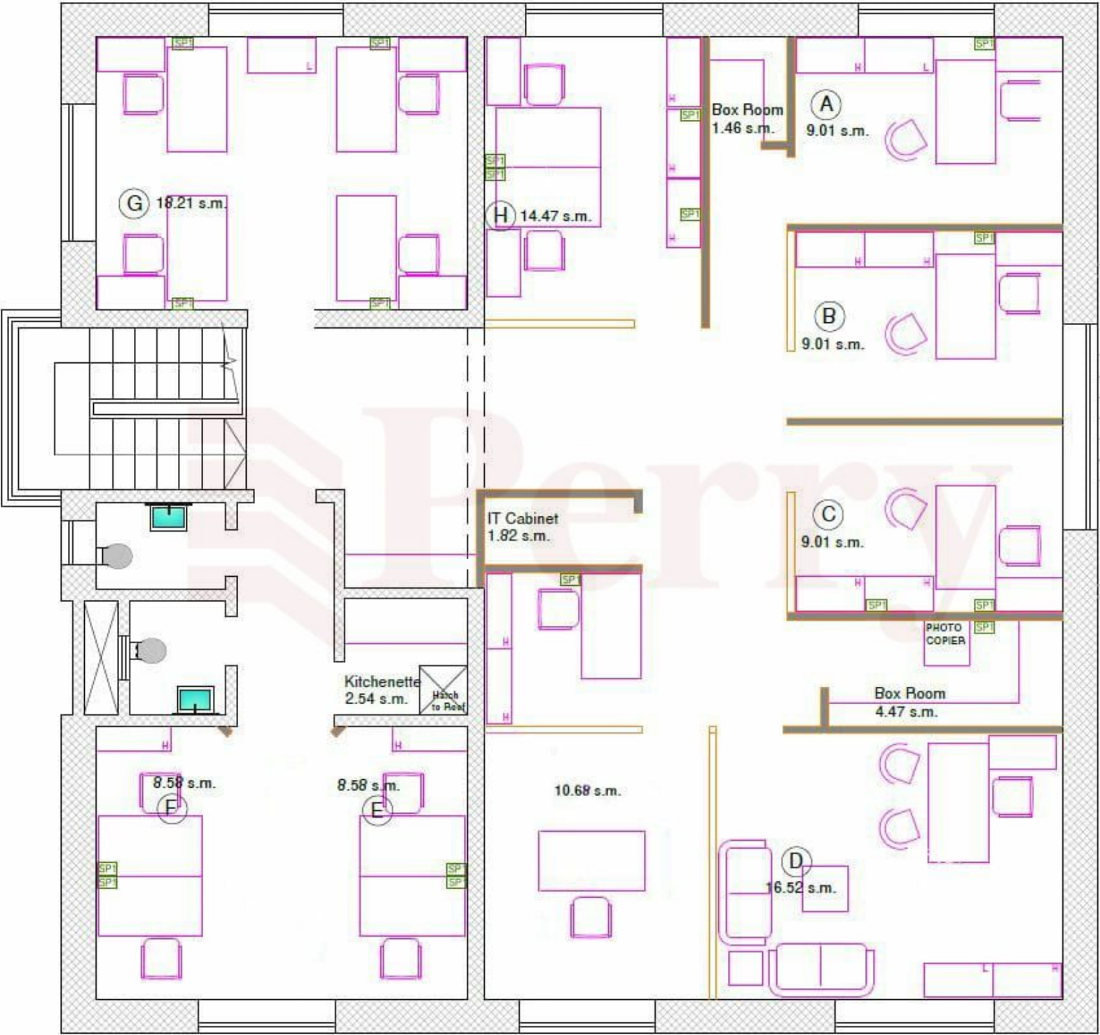
SECOND FLOOR PLAN 168.17 s.m.
