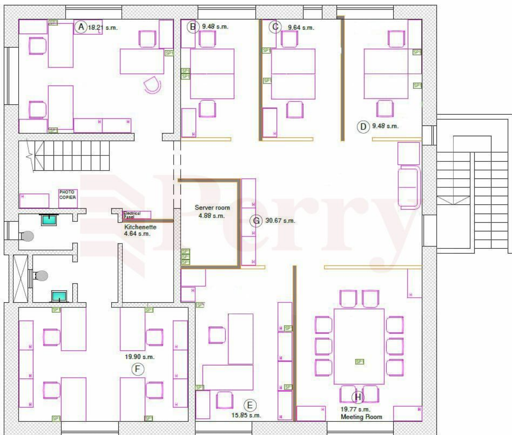
FIRST FLOOR PLAN 165.85 s.m.
