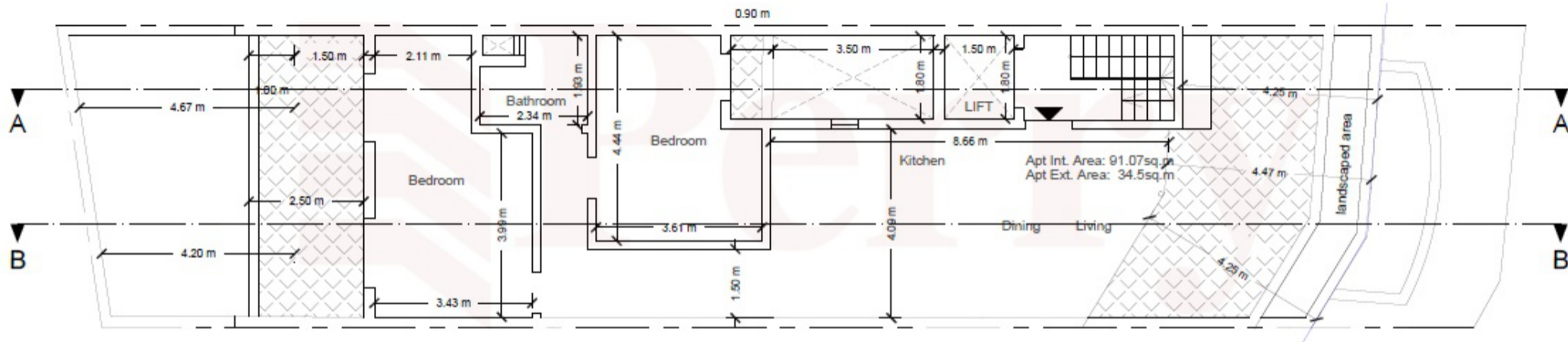
EXISTING RECEDED FLOOR LEVEL PLAN
