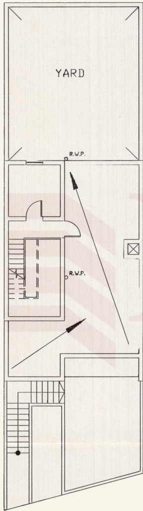
EXISTING SECOND FLOOR
